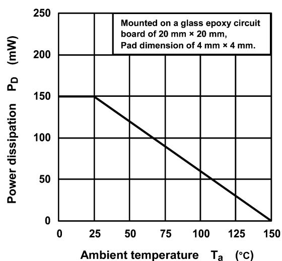
Fig. 7.4 P_D - T_a
