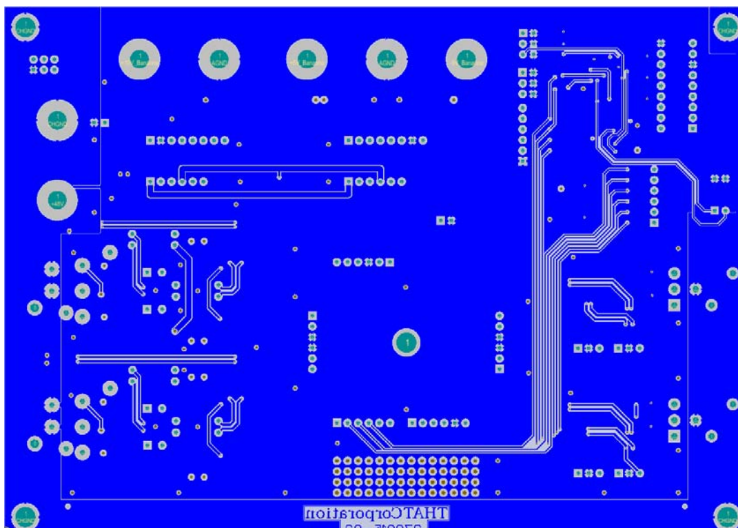
Mother Board, Bottom Layer
