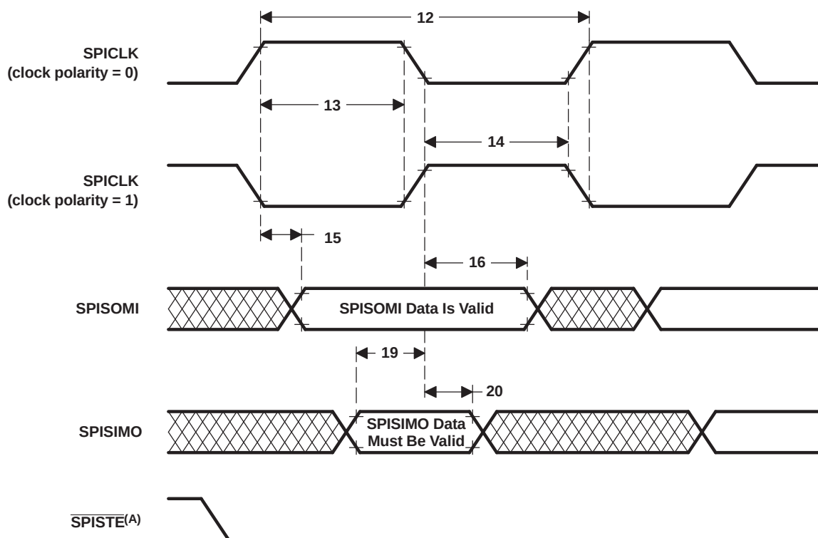
Figure 5-19. SPI Slave Mode External Timing (Clock Phase = 0)
