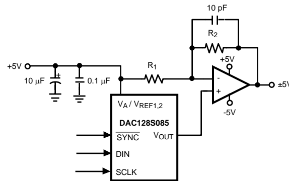
Figure 36. Bipolar Operation
