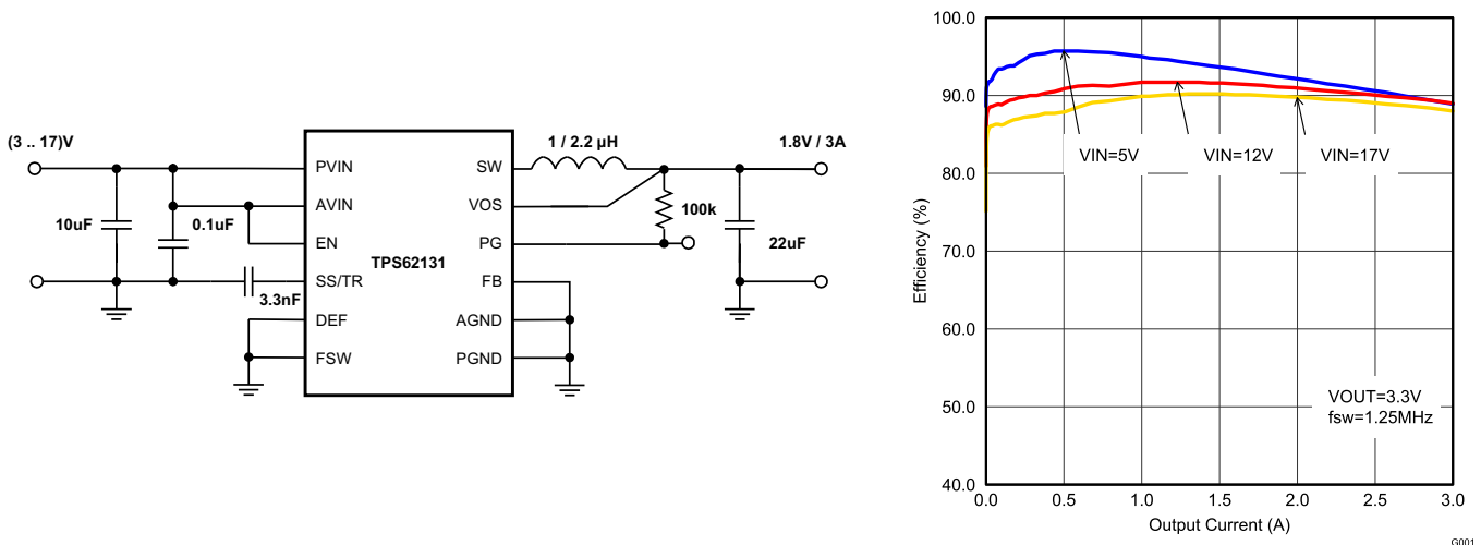
Figure 1. Typical Application and Efficiency
