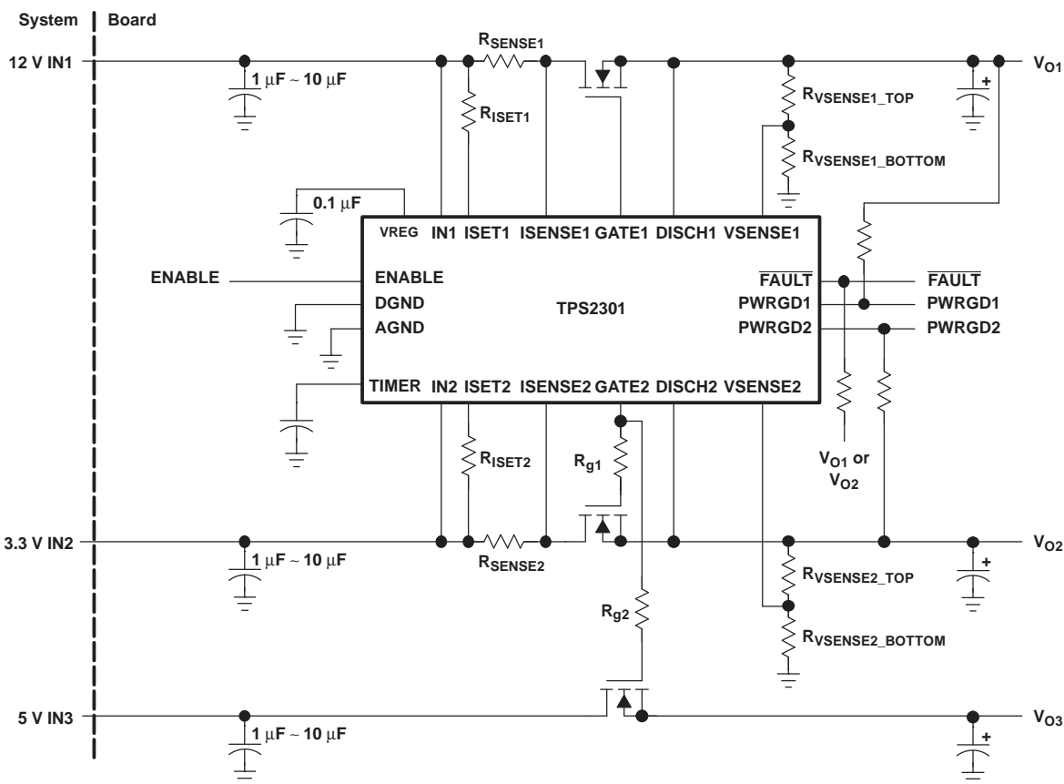
Figure 28. Three-Channel Application
