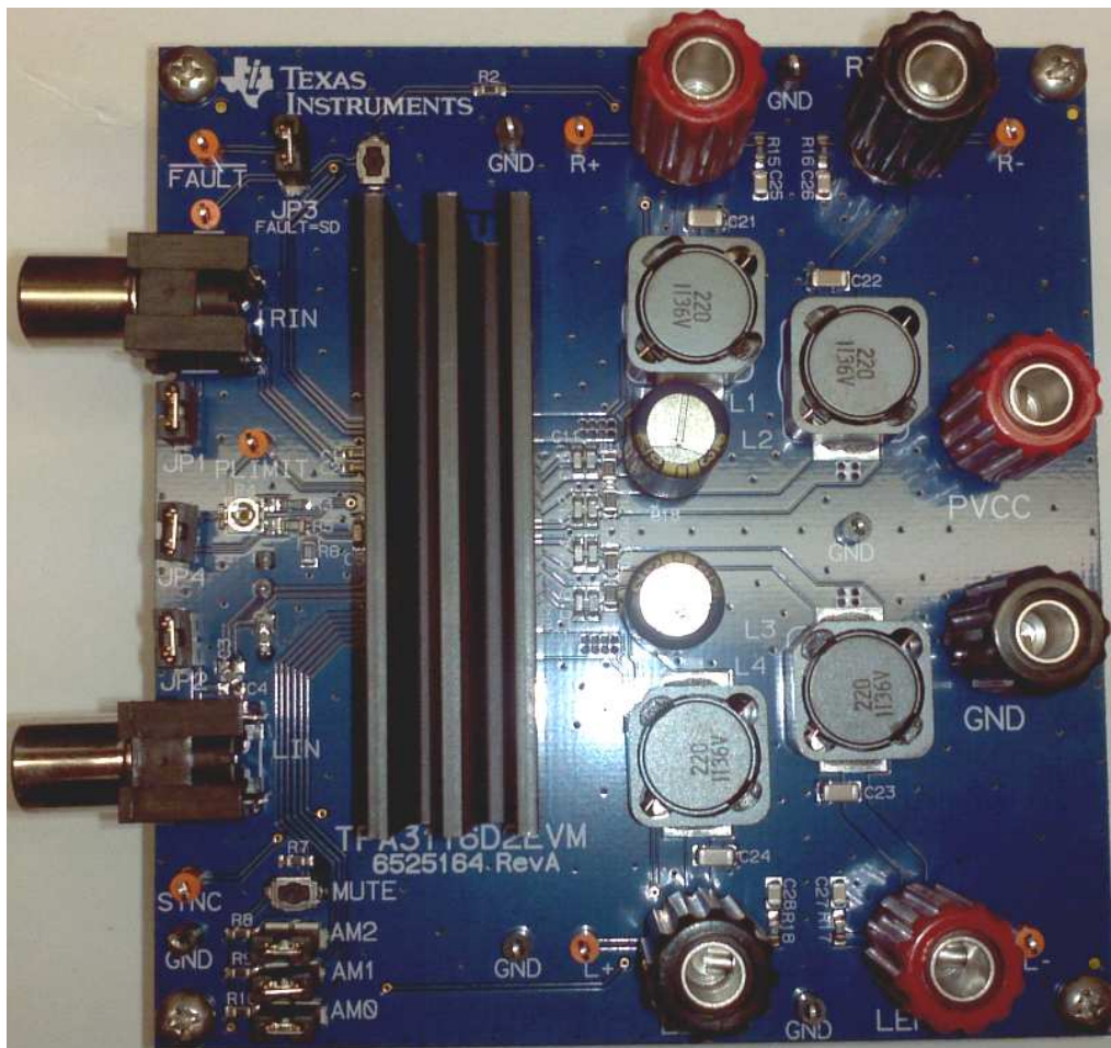
Figure 1. TPA3116D2EVM Evaluation Module
