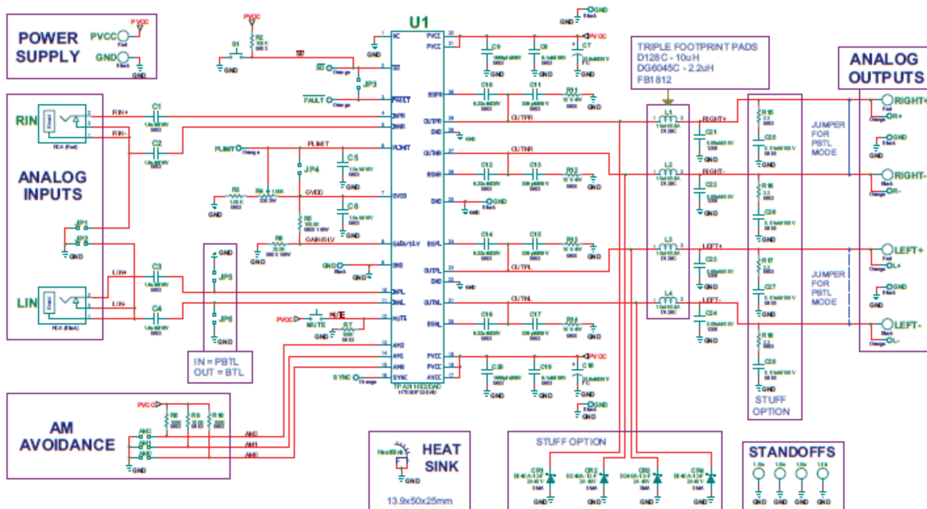
Figure 2. TPA3116D2EVM Schematic
