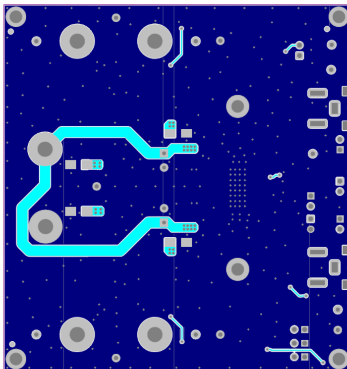
Figure 4. TPA3116D2EVM Bottom-Side Layout
