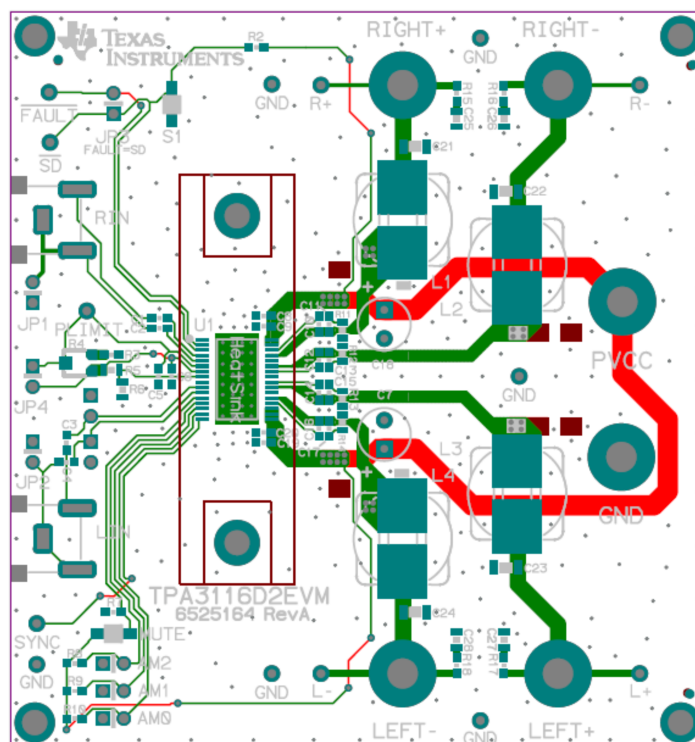
Figure 5. TPA3116D2EVM Top X-Ray View
