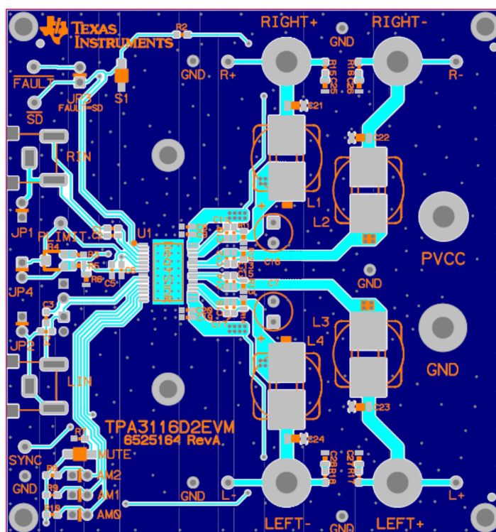
Figure 3. TPA3116D2EVM Top-Side Layout
