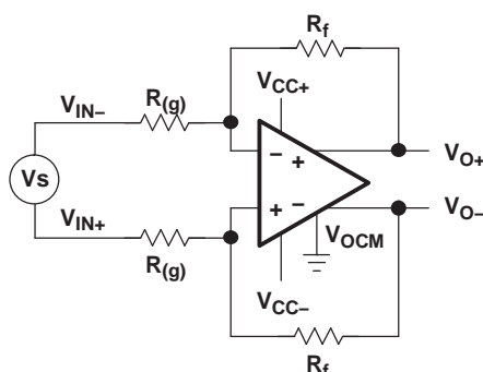
Figure 38. Amplifying Differential Signals
