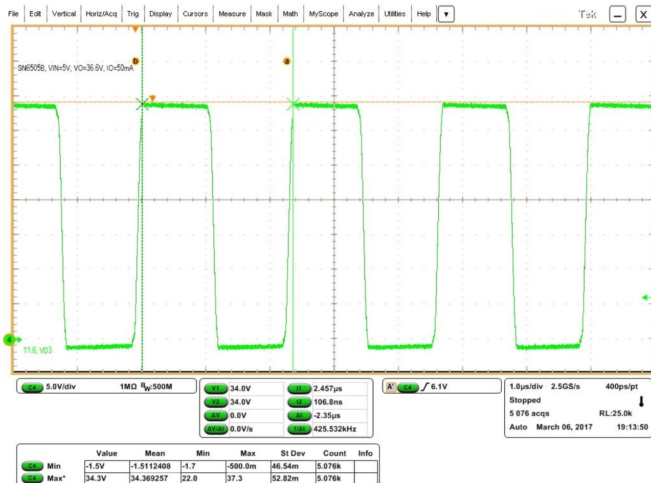
Figure 17. Bias Supply Secondary Side Switching Waveforms
