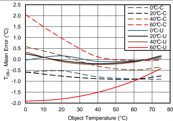
Figure 19. Mean Calibration Error, Wide Range Over T DIE
