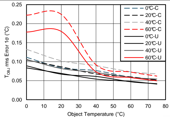
Figure 20. Noise in Temperature Measurement, Wide Range Over T DIE
