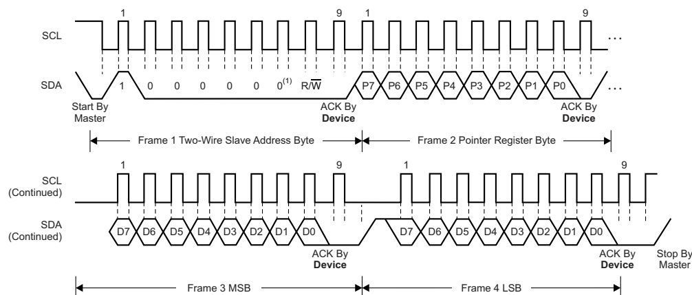
Figure 11. Two-Wire Timing Diagram For Write Word Format
