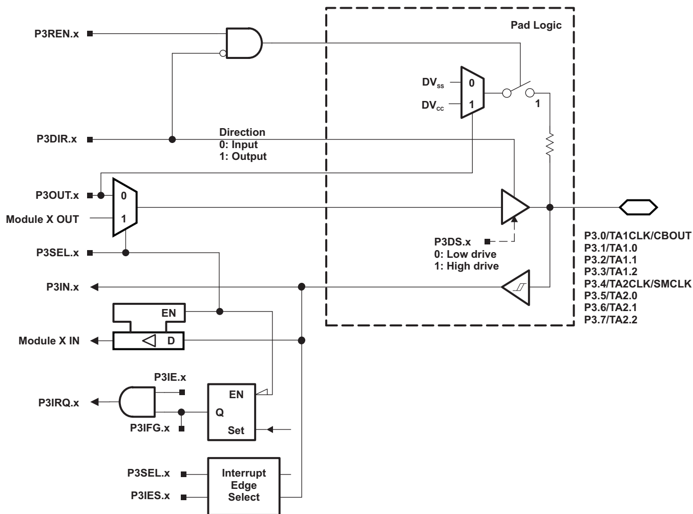
Figure 6-4. Port P3 (P3.0 to P3.7) Schematic
