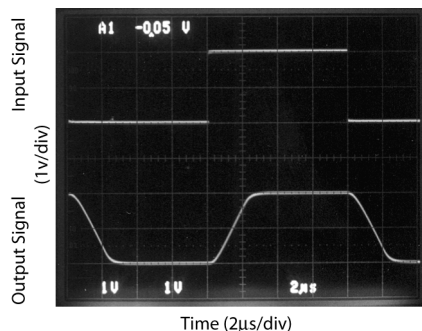
Figure 50. Pulse Response of the LMV324 Circuit in Figure 49
