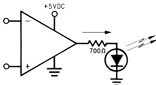
Figure 70. LED Driver
