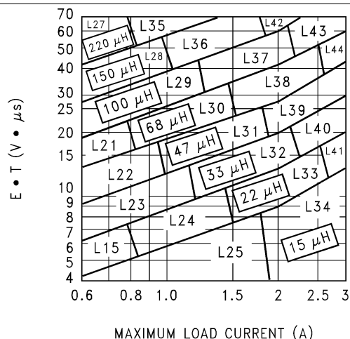
Figure 30. LM2596-ADJ
