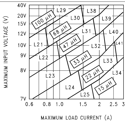
Figure 28. LM2596-5.0
