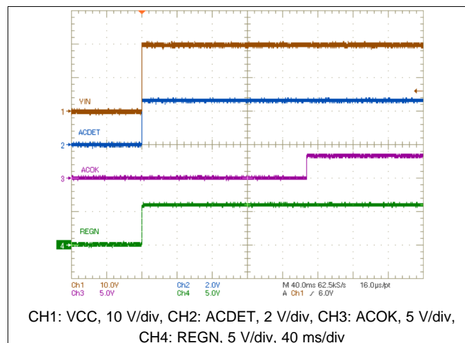
Figure 1. VCC, ACDET, REGN and ACOK Power Up
