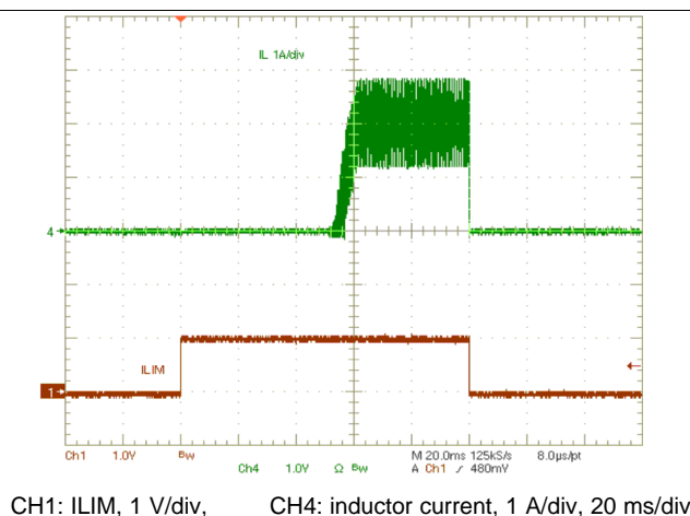
Figure 2. Charge Enable by ILIM
