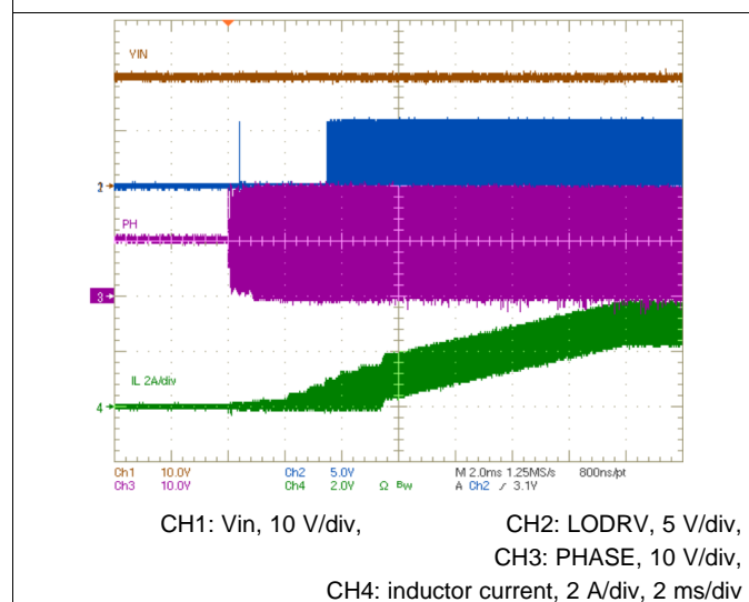
Figure 3. Current Soft-Start
