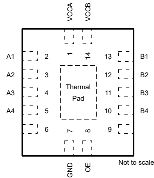
Figure 4-1. BQA Package, 14-Pin WQFN (Top View)
