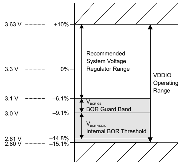
Figure 6-10. Supply Voltages
