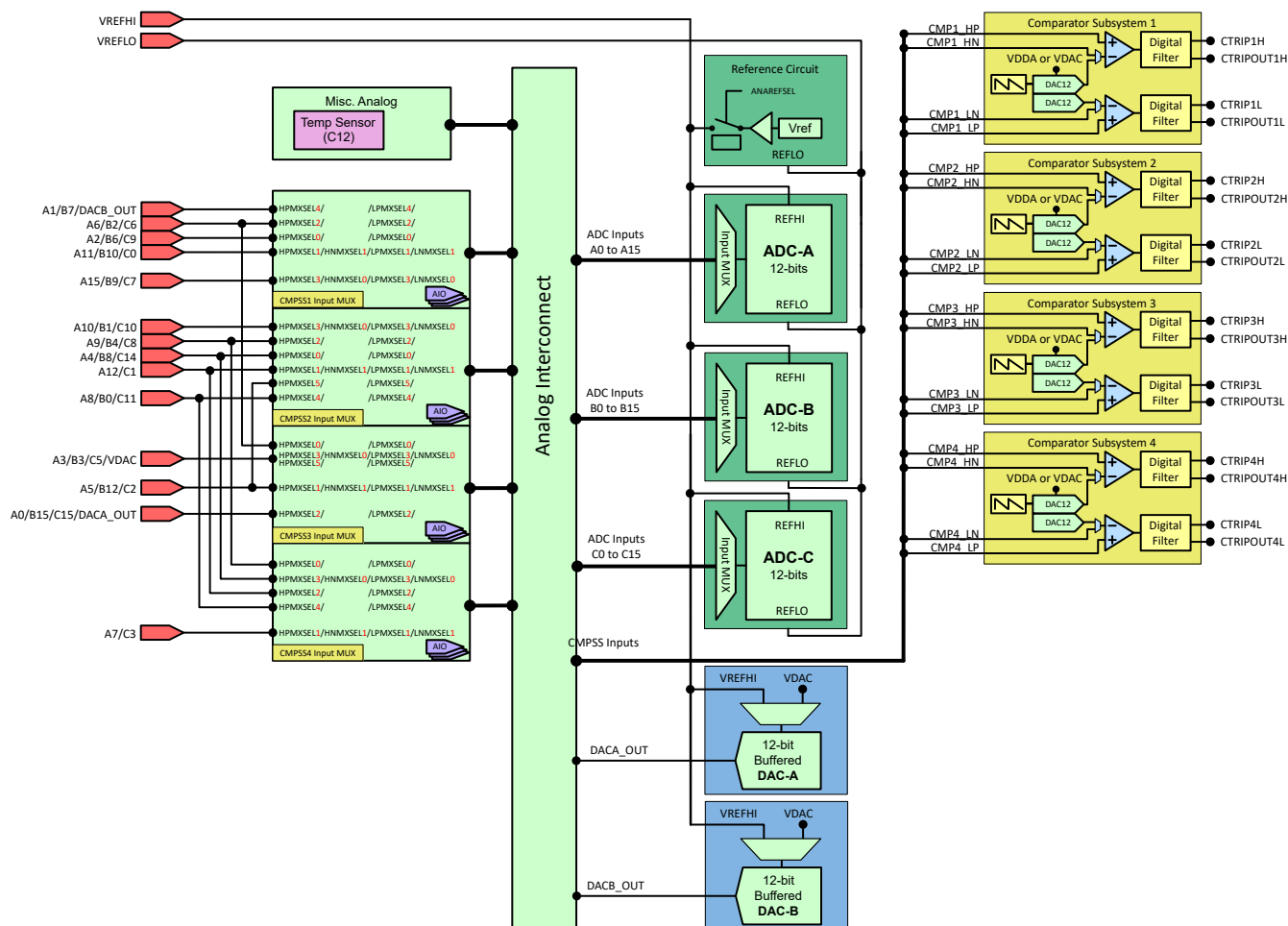
Figure 6-40. Analog Subsystem Block Diagram (48-Pin PT LQFP)
