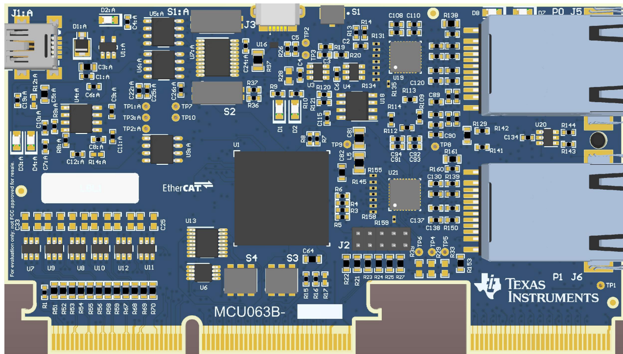
Figure 1. F28388D controlCARD
