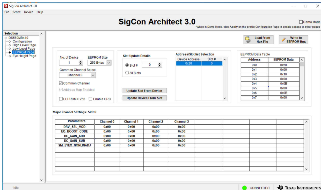
Figure 5-11. EEPROM Page
