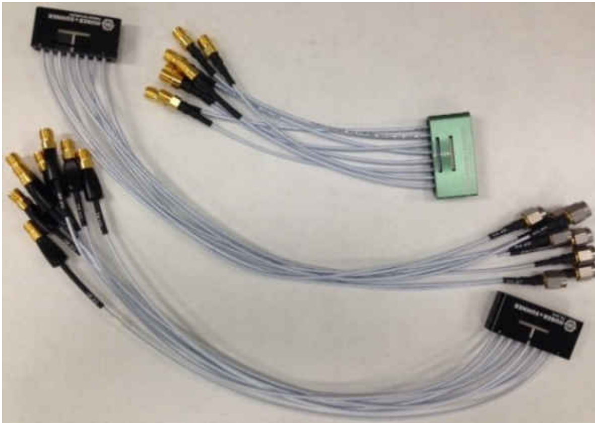
Figure 8-1. Huber+Suhner 1x8 MXP Cable Assemblies
