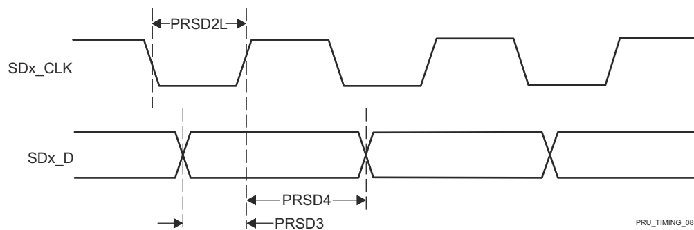
Figure 7-95. PRU_ICSSG PRU SD_CLK Rising Active Edge
