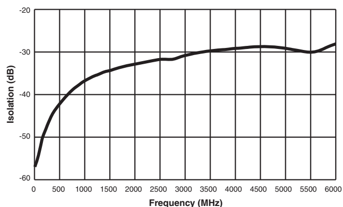
Isolation Pole to Pole (RF Note 5)
