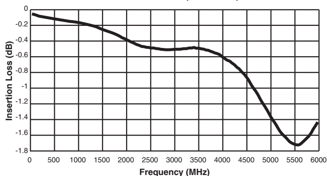
Insertion Loss (RF Note 6)
