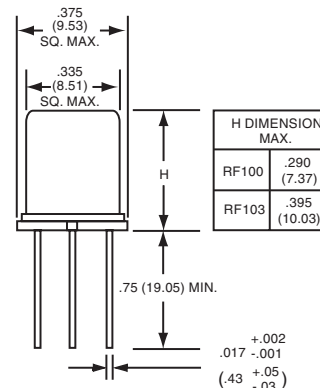
EXTERNAL DIMENSIONS
