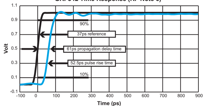
GRF342 Time Response (RF Note 6)
