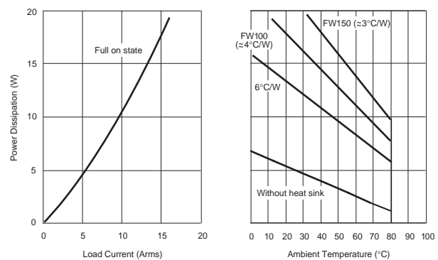
Figure 4 — LS relays
