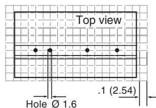
Figure 12 — LS relays with HS1; dimensions in inches (mm)
