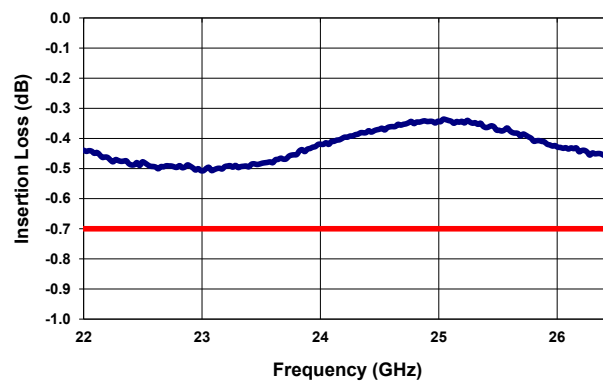
Insertion Loss ( 22-26.5 GHz )
