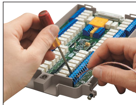
Screw terminals use oversized connectors for easier, mistake-free wiring. Easy-to-use removable terminals are available on some models.
