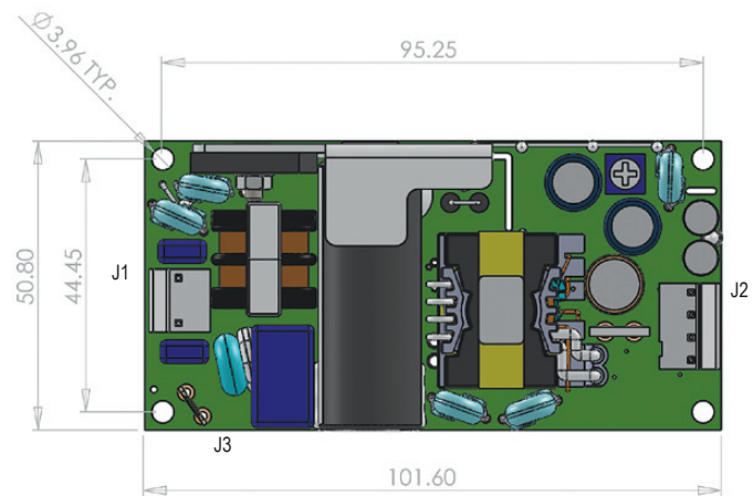
Outline Drawing ZMS100 12 - 15V Series
