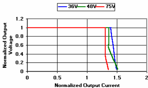
X1048S03,S05 V/I Characteristic at 25C
