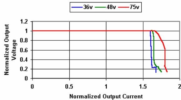
X2048S03,S05 V/I Characteristic at 25C
