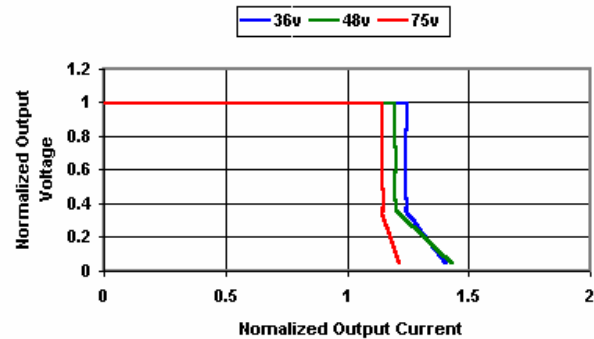
X1048S03,S05 V/I Characteristic at 70C
