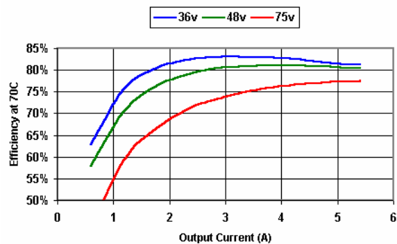
X2048S2.5 Efficiency at 70C
