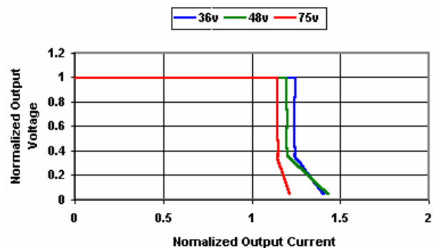
X1048S03,S05 V/I Characteristic at 70°C
