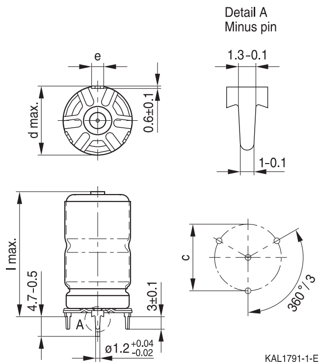
Soldering star capacitors, 3-pin design
