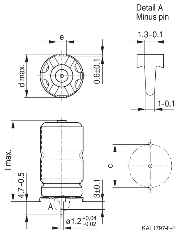
Soldering star capacitors, 2-pin design
