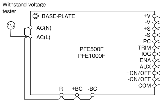
2.5kVAC 1 minute (20mA) Fig. 21-1 Input to Baseplate Withstand Voltage Test Method
