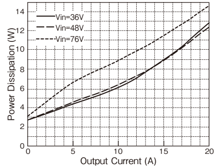
Fig.1-8 PAQ100S48-5/B Power dissipation vs Output Current (Output voltage: Nominal, T_a=60^\circ C ; typical value)
