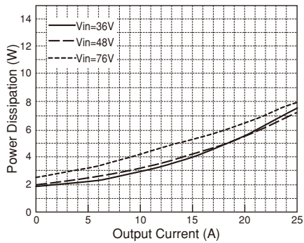
Fig.1-5 PAQ100S48-1R8/B Power dissipation vs Output Current (Output voltage: Nominal, T_a=60^\circ C ; typical value)
