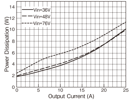
Fig.1-6 PAQ100S48-2R5/B Power dissipation vs Output Current (Output voltage: Nominal, T_a=60^\circ C ; typical value)
