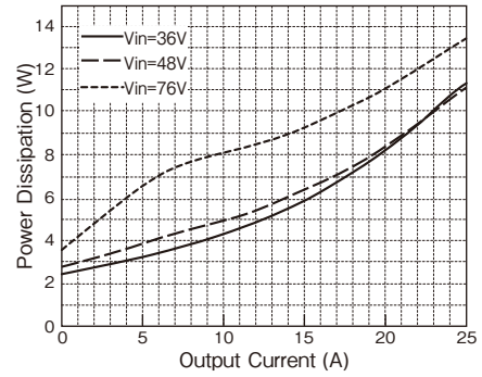
Fig.1-7 PAQ100S48-3R3/B Power dissipation vs Output Current (Output voltage: Nominal, T_a=60^\circ C ; typical value)
