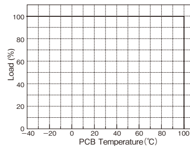
Fig.1-13 Output Derating by PAQ100S48 PCB Temperature
