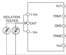
Fig.18-1: Isolation test
