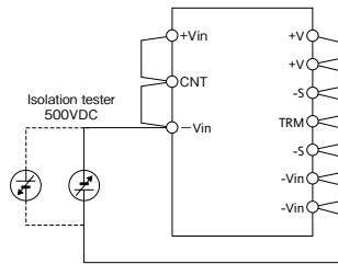
100M \Omega and above at 500VDC Fig.20-1 Isolated test
