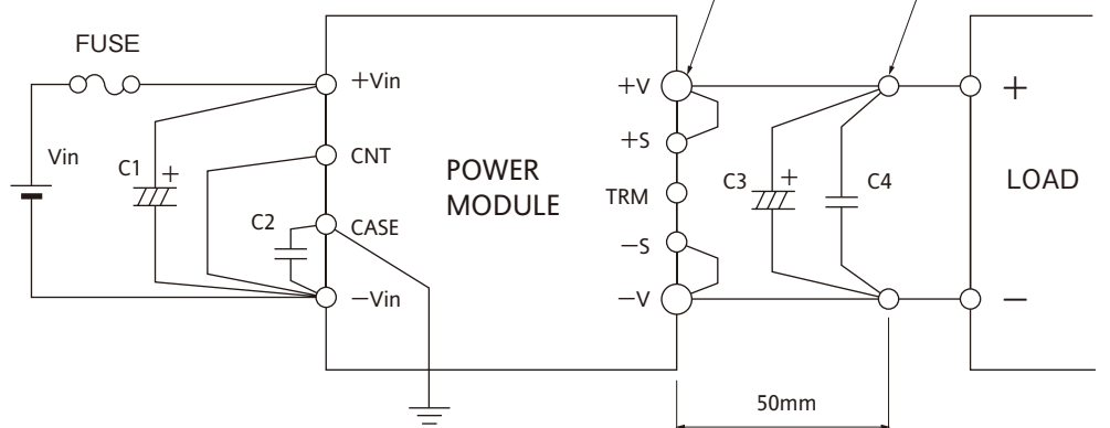
Basic connection
