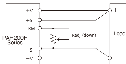
Fig.2-2 Connection for output voltage trim down (1)
