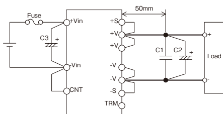
Fig.1-2 Basic Connection
