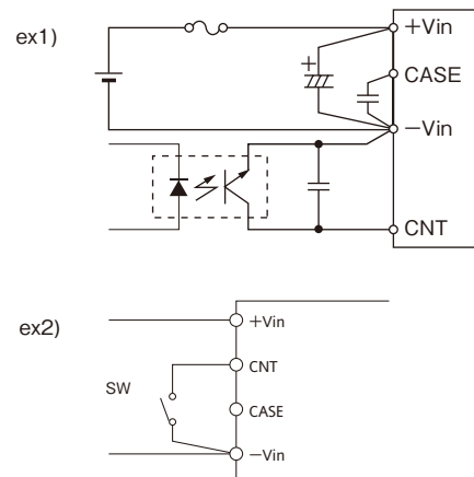
CNT Connection Method
