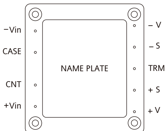
Basic connection
