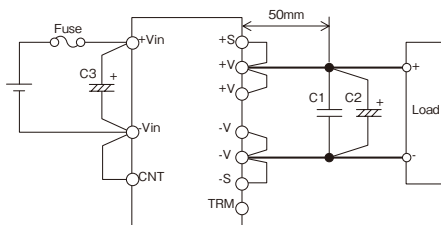
Fig.1-2 Basic Connection
