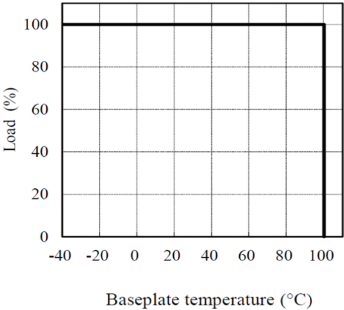
Derating Curve (PH50A to PH300A)
