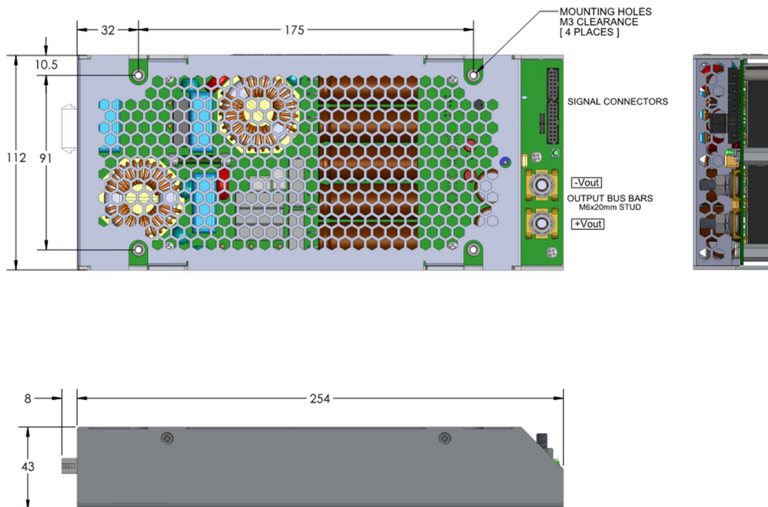
Fig 28-1: Dimensions for Standard and /C chassis configurations
