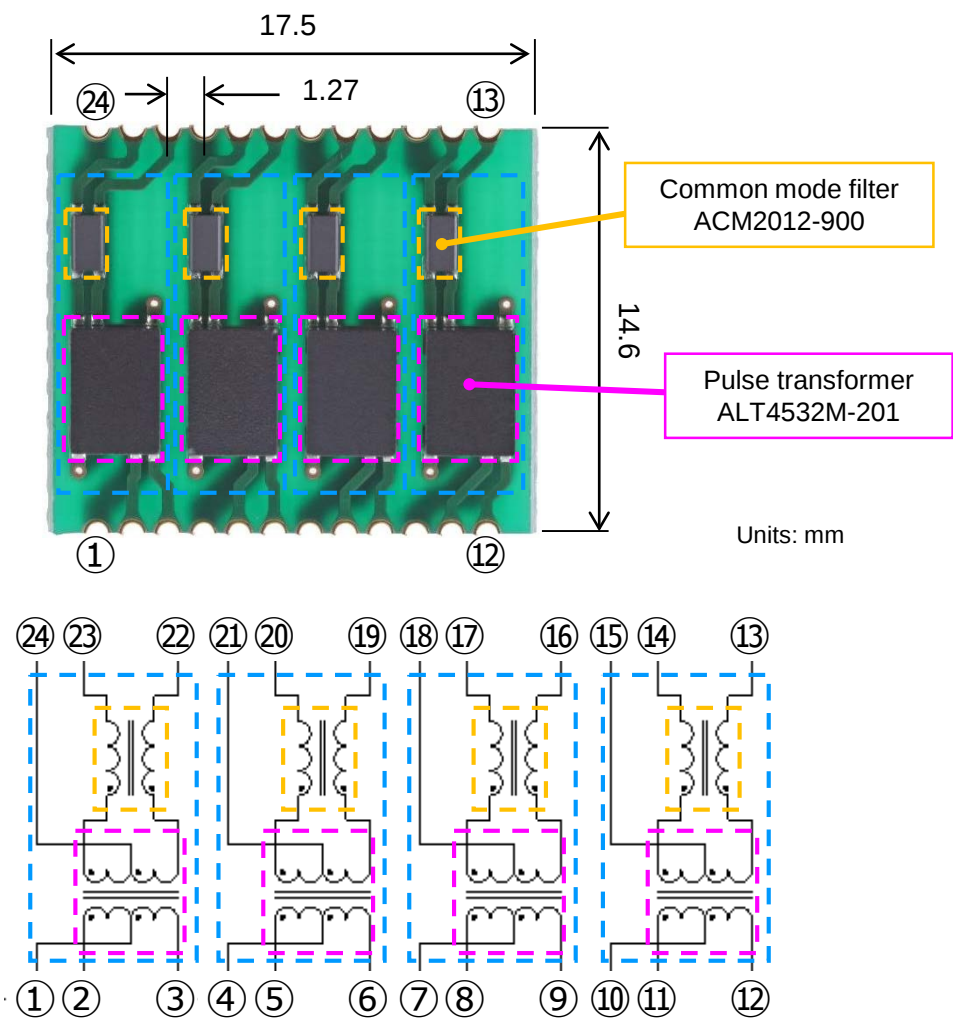
Evaluation Board Electrical diagram and pin out
