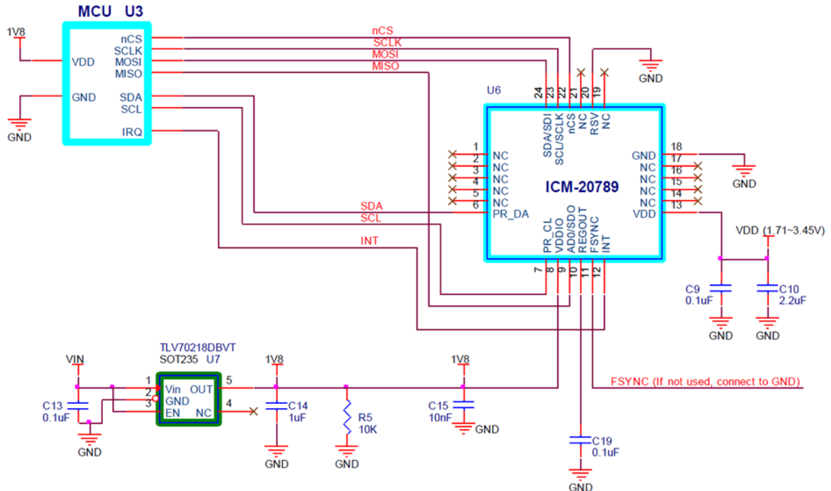
SPI Communication for Gyro/Accel; I 2 C Pressure; MCU Digital Interface: 1.8V Schematic
