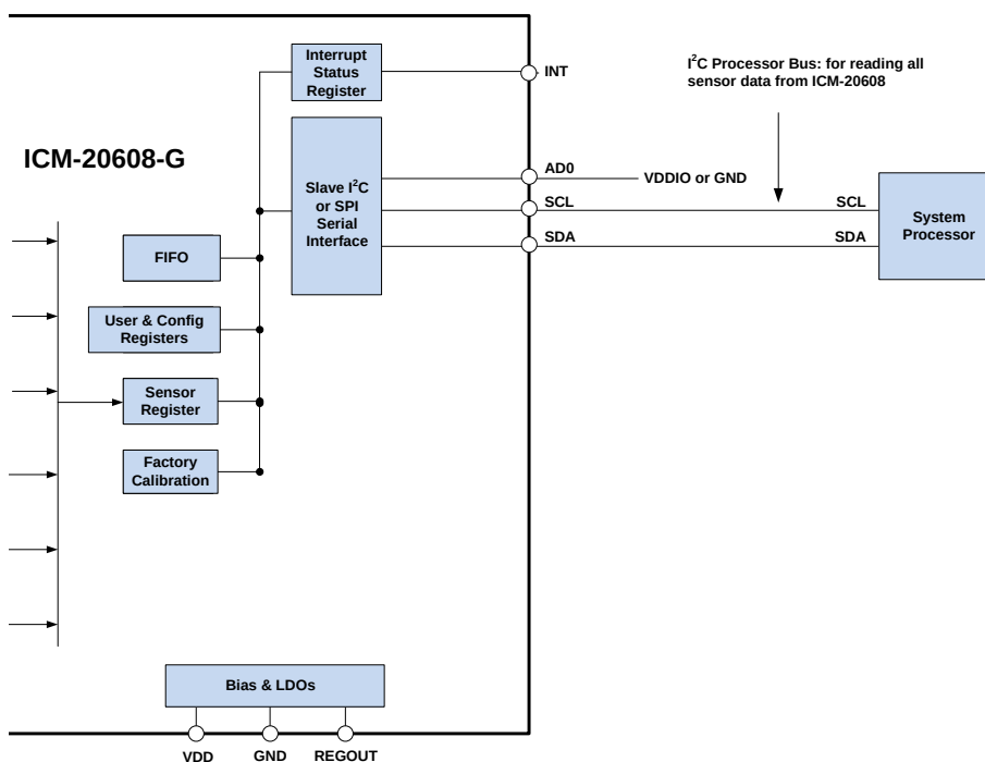
Figure 7. ICM-20608-G Solution Using I²C Interface
