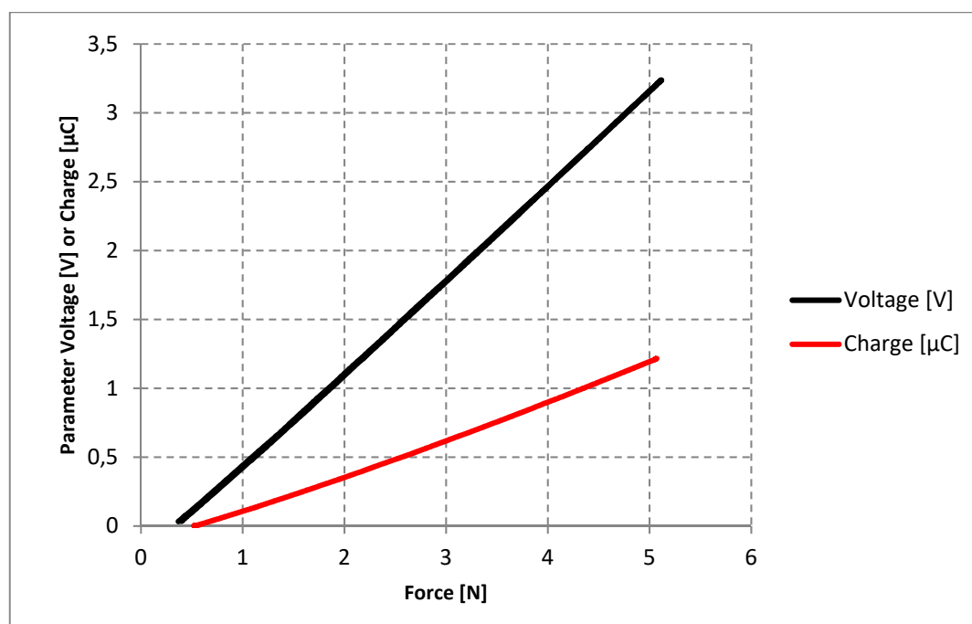
Fig. 10: Sensor characteristics open circuit voltage or short circuit charge as a function of force input.
