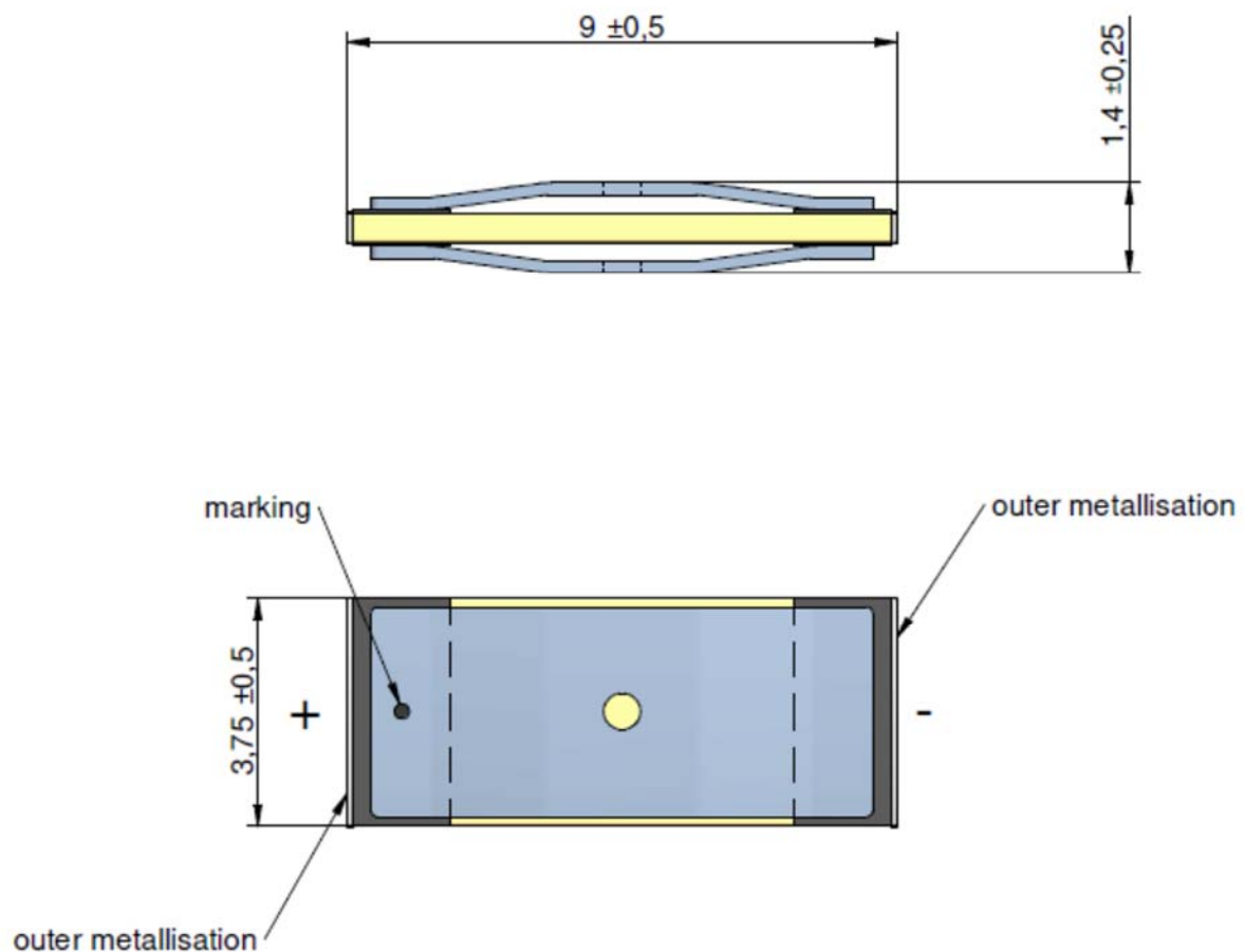
Fig. 1: Dimensional Drawing
