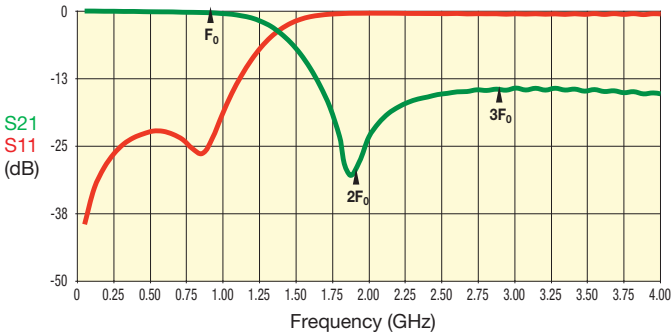
LP0603A0947ANTR
