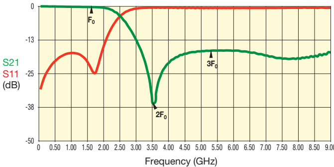
LP0603A1747ANTR
