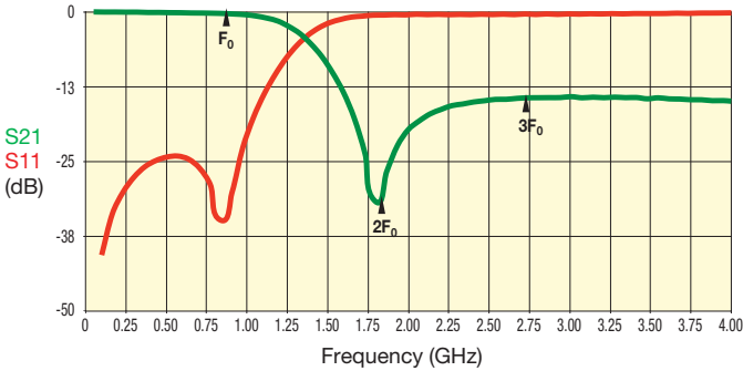
LP0603A0902ANTR
