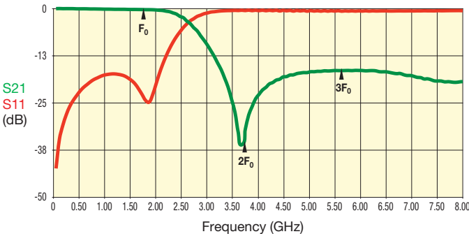
LP0603A1842ANTR
