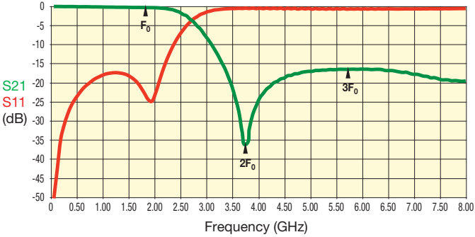
LP0603A1880ANTR
