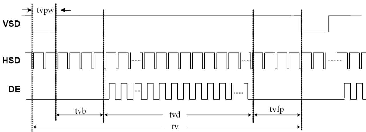
Figure 8 Vertical timing
