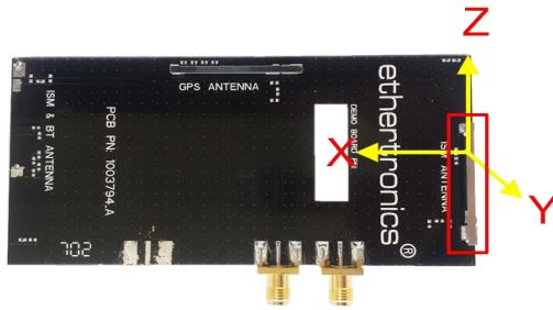
Single Band antenna (ISM Layout Orientation)
