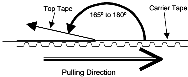
Fig.9 Peeling Strength
