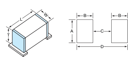
MOUNTING PAD DIMENSIONS CASE CL, CS & CF: inches (millimeters)
