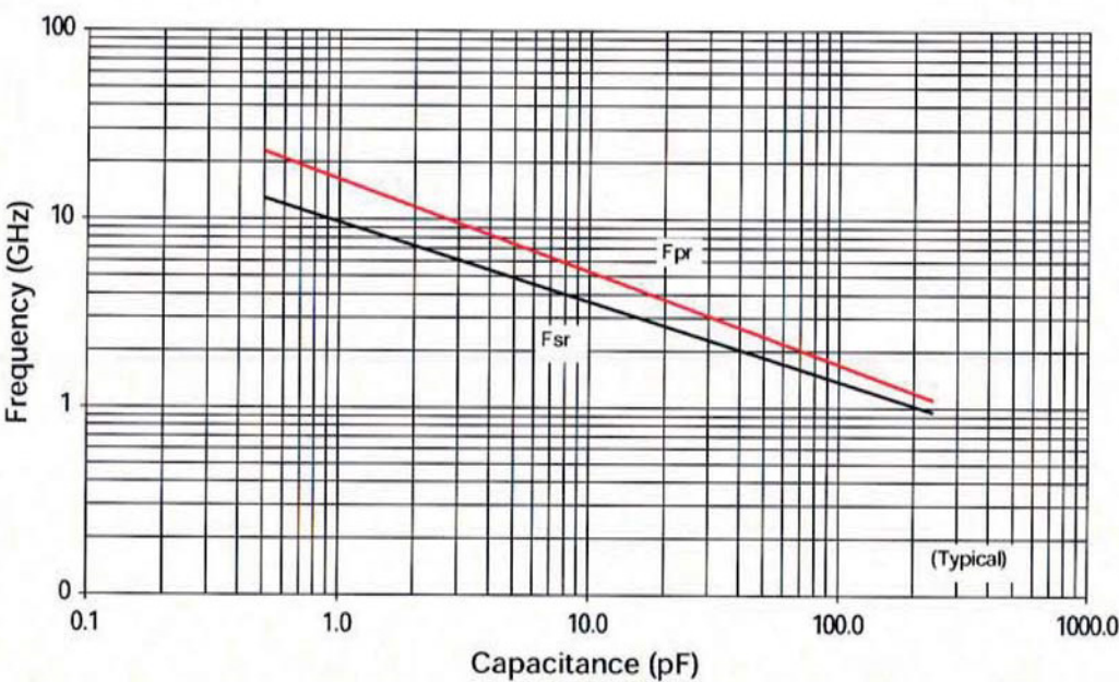
UQ CF Resonant Frequency
