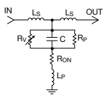
Electrical Model
