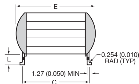
LEAD STYLE L AND B
