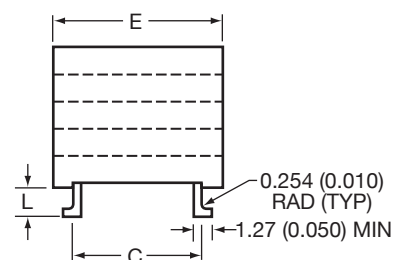
LEAD STYLE L AND B
