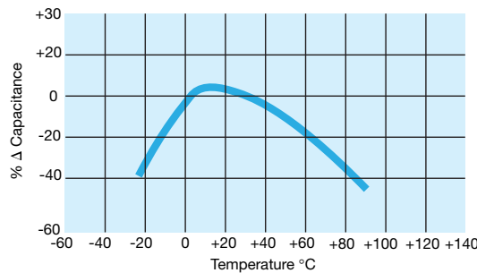
Temperature Coefficient
