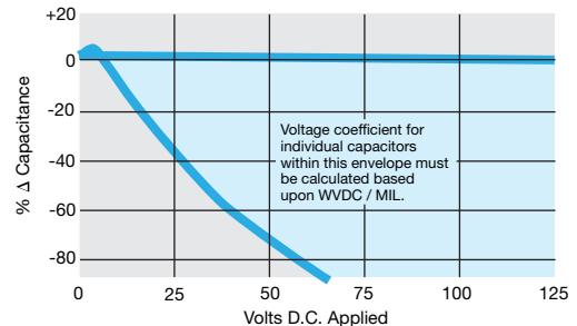
Voltage Coefficient
