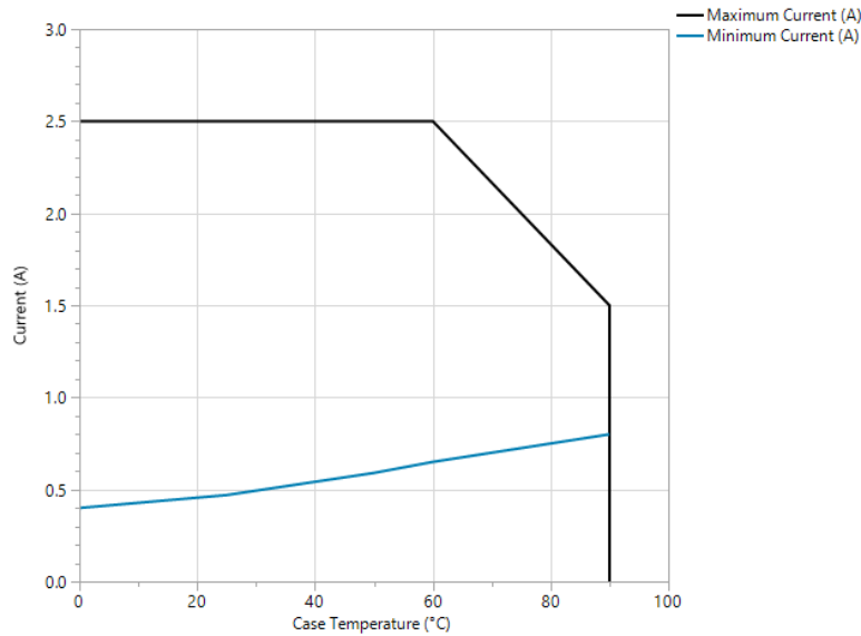
Figure 05: Maximum and minimum current vs temperature to maintain performance and lifetime of component. Operating below minimum current will result in near zero light output.
