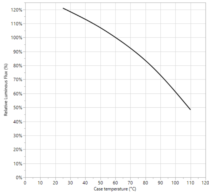
Figure 04: Relative luminous flux vs case temperature (Normalized luminous flux at I_f = 2.5\text{A} and at T_{\text{case}} = 60^\circ\text{C} )
