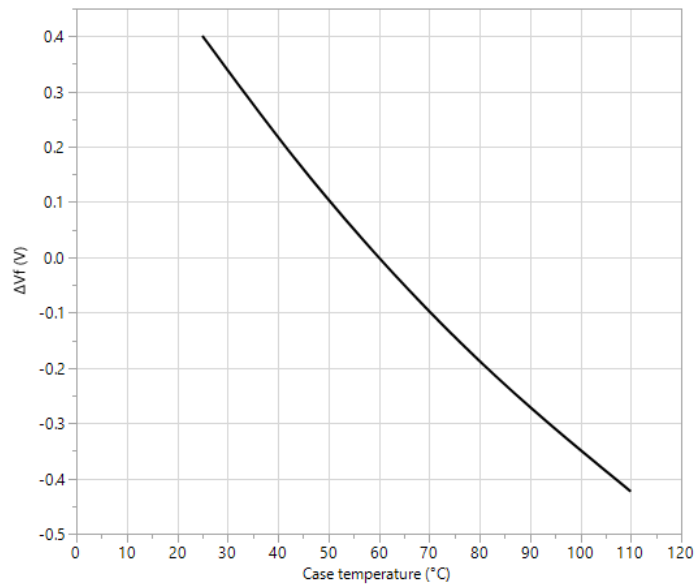
Figure 06: Forward voltage vs temperature (Measured at I_f = 2.5A and normalized at T_{case} = 60^\circ C )
