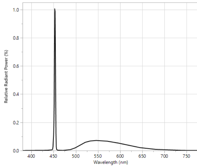
Figure 02: Typical spectral power distribution of 6500K component ( I_f = 2.5A , T_{case} = 60^{\circ}C )
