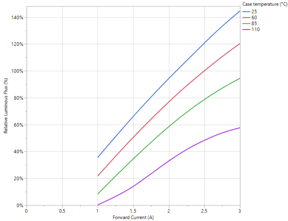
Figure 03: Relative flux vs forward current (Normalized to at I_f = 2.5\text{A} and T_{\text{case}} = 60^\circ\text{C} )
