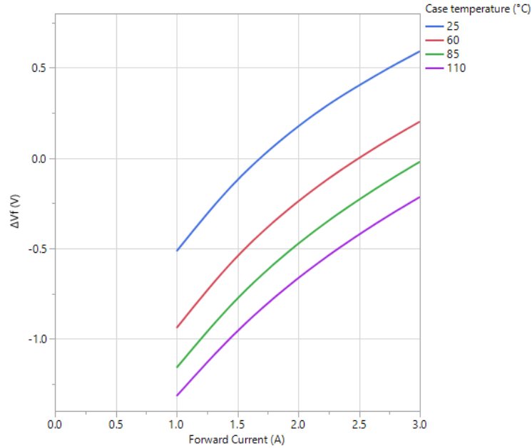
Figure 07: Change in forward voltage vs forward current (Normalized to at I_f = 2.5\text{A} and T_{\text{case}} = 60^\circ\text{C} )
