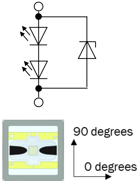
Figure 9: Orientation for near and far field plots
