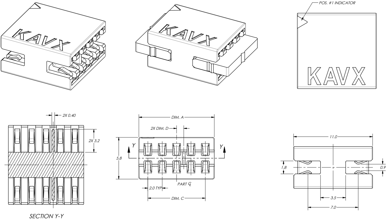
SECTION Y-Y
