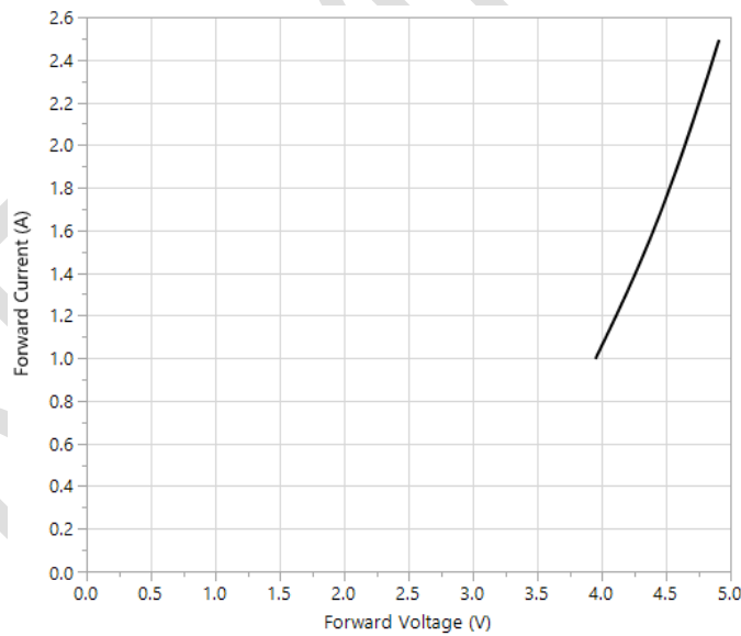
Figure 07: White channel: forward current vs forward voltage (Measured at T_{\text{case}} = 50^\circ\text{C} )
