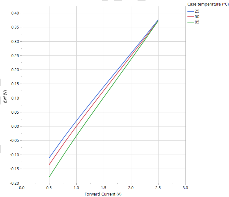
Figure 11: IR channel: change in forward voltage vs forward current (Normalized to at I_f = 1.0A and T_{case} = 50^\circ C )
