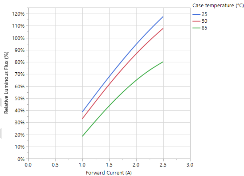
Figure 05: White channel: relative luminous flux vs current (Normalized luminous flux at I_f = 2.3\text{A} and at T_{\text{case}} = 50^\circ\text{C} )
