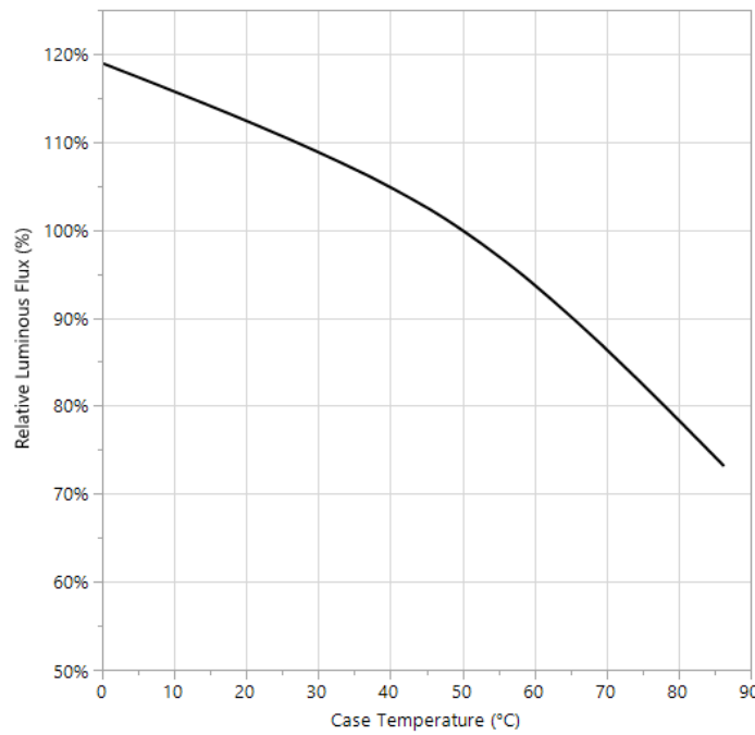
Figure 08: White channel: relative luminous flux vs case temperature (Normalized luminous flux at I_f = 2.3A and at T_{case} = 50^{\circ}C )
