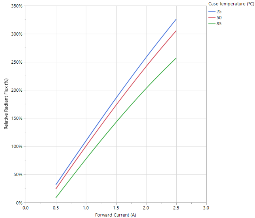
Figure 10: IR channel: relative radiant flux vs current (Normalized luminous flux at I_f = 1.0A and at T_{case} = 50^\circ C )
