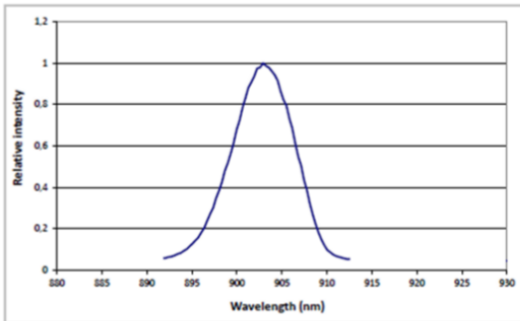
Figure 03: Typical spectral power distribution of 905nm IR channel (IR channel measured at I_f = 1.0A , T_{case} = 50^{\circ}C )
