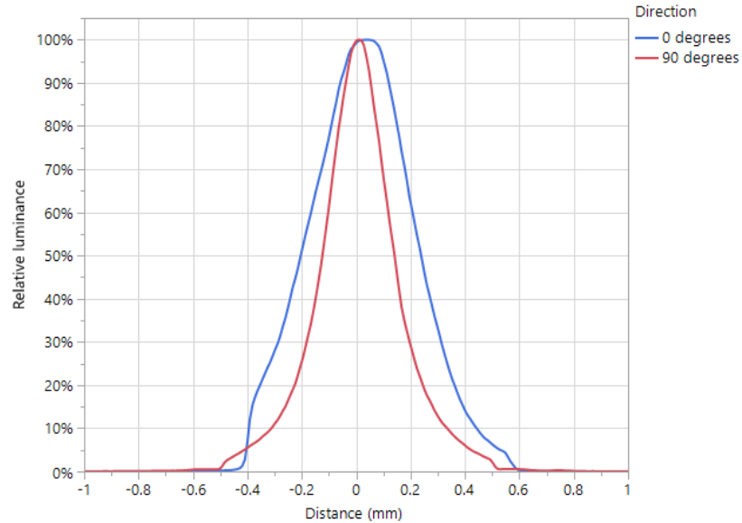
Figure 20: White channel: near field relative luminance (Measured at I_f = 2.3A and at T_{case} = 50^{\circ}C , normalized to 0,0 position)
