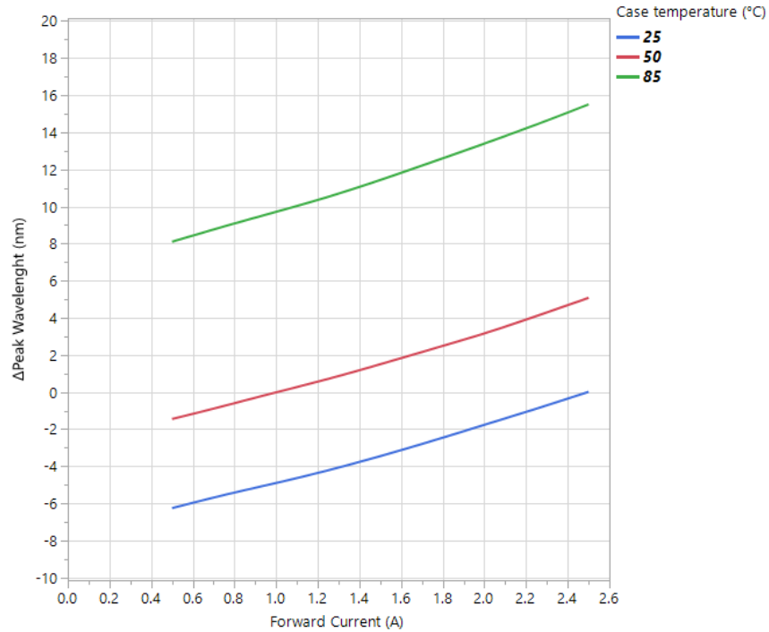
Figure 14: IR channel: Change in peak wavelength vs forward current (Peak wavelength normalized at I_f = 1.0A and at T_{case} = 50^\circ C )
