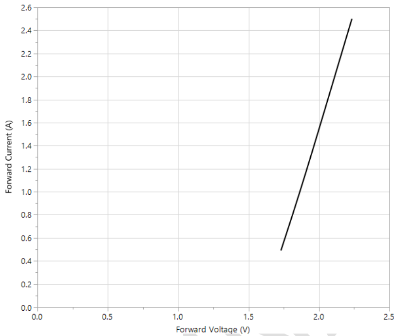
Figure 12: IR channel: forward current vs forward voltage (Measured at T_{\text{case}} = 50^{\circ}\text{C} )
