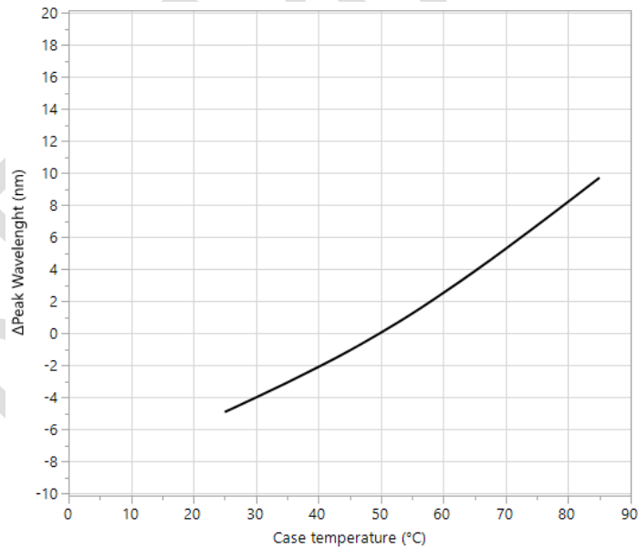
Figure 15: IR channel: Change in peak wavelength vs case temperature (Peak wavelength normalized at I_f = 1.0A and at T_{case} = 50^\circ C )
