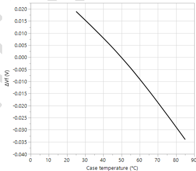
Figure 09: IR channel: change in forward voltage vs temperature (Measured at I_f = 1.0A and normalized at T_{case} = 50^{\circ}C )
