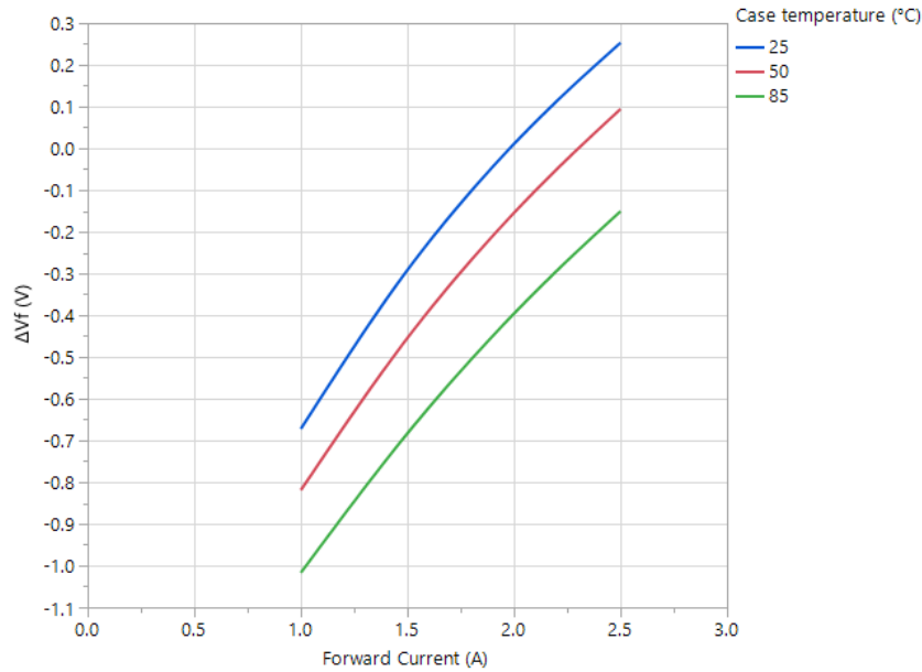
Figure 06: White channel: change in forward voltage vs forward current (Normalized to at I_f = 2.3\text{A} and T_{\text{case}} = 50^\circ\text{C} )
