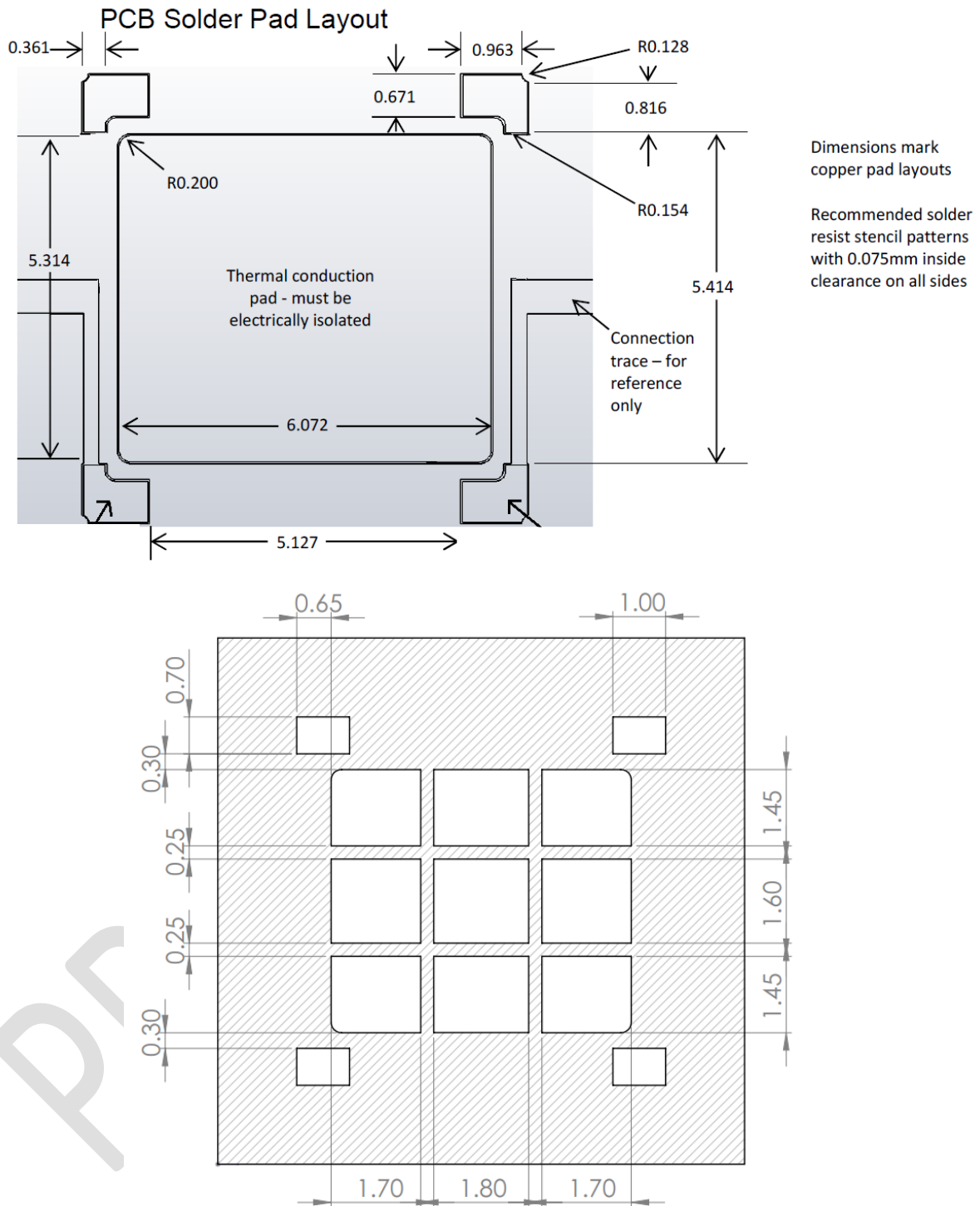
Figure 16: Recommended stencil mask design
