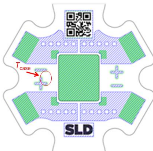
Figure 22: Recommended location of T_{case} measurement
