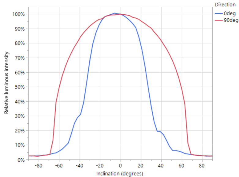
Figure 18: White channel: far field distribution (Measured at I_f = 2.3A and at T_{case} = 50^{\circ}C , normalized to 0,0 position)
