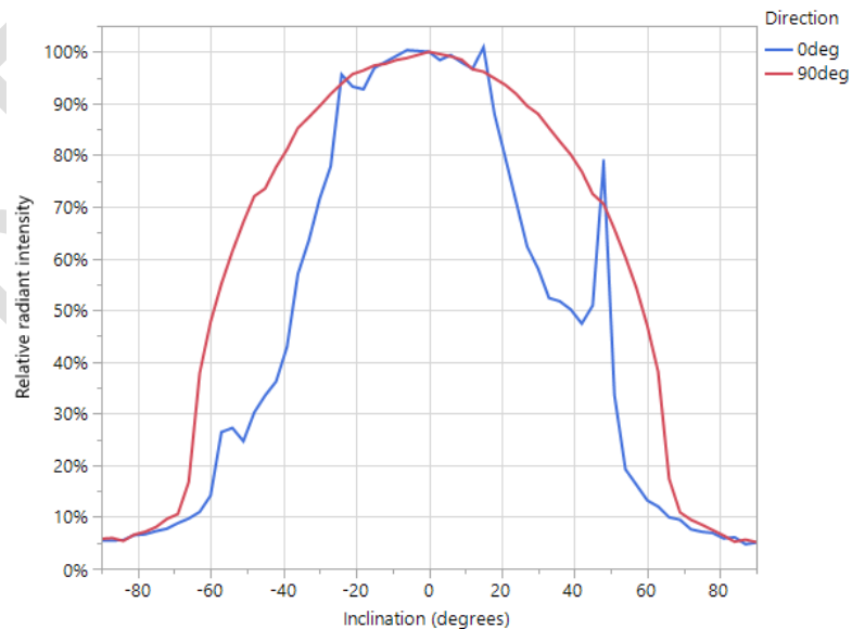
Figure 19: IR channel: far field distribution (Measured at I_f = 1.0A and at T_{case} = 50^{\circ}C , normalized to 0,0 position)
