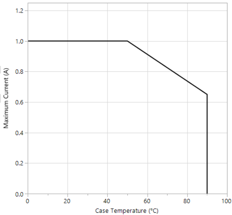
Figure 24: Derating curve for IR channel
