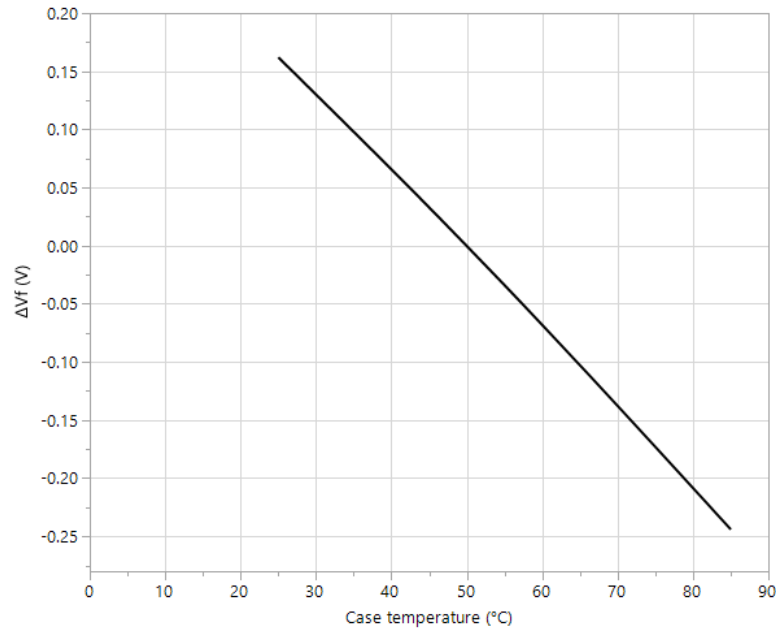
Figure 04: White channel: change in forward voltage vs temperature (Measured at I_f = 2.3\text{A} and normalized at T_{\text{case}} = 50^\circ\text{C} )
