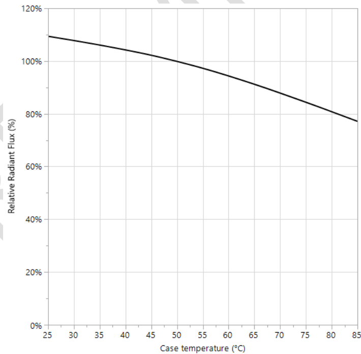
Figure 13: IR channel: relative radiant flux vs case temperature (Normalized luminous flux at I_f = 1.0\text{A} and at T_{\text{case}} = 50^{\circ}\text{C} )
