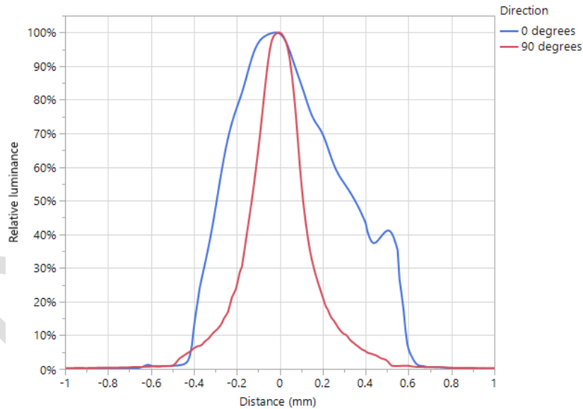
Figure 21: IR channel: near field relative luminance (Measured at I_f = 1.0A and at T_{case} = 50^{\circ}C , normalized to 0,0 position)
