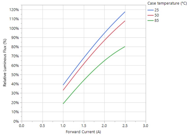
Figure 04: White channel: relative luminous flux vs current (Normalized luminous flux at I_f = 2.3\text{A} and at T_{\text{case}} = 50^\circ\text{C} )
