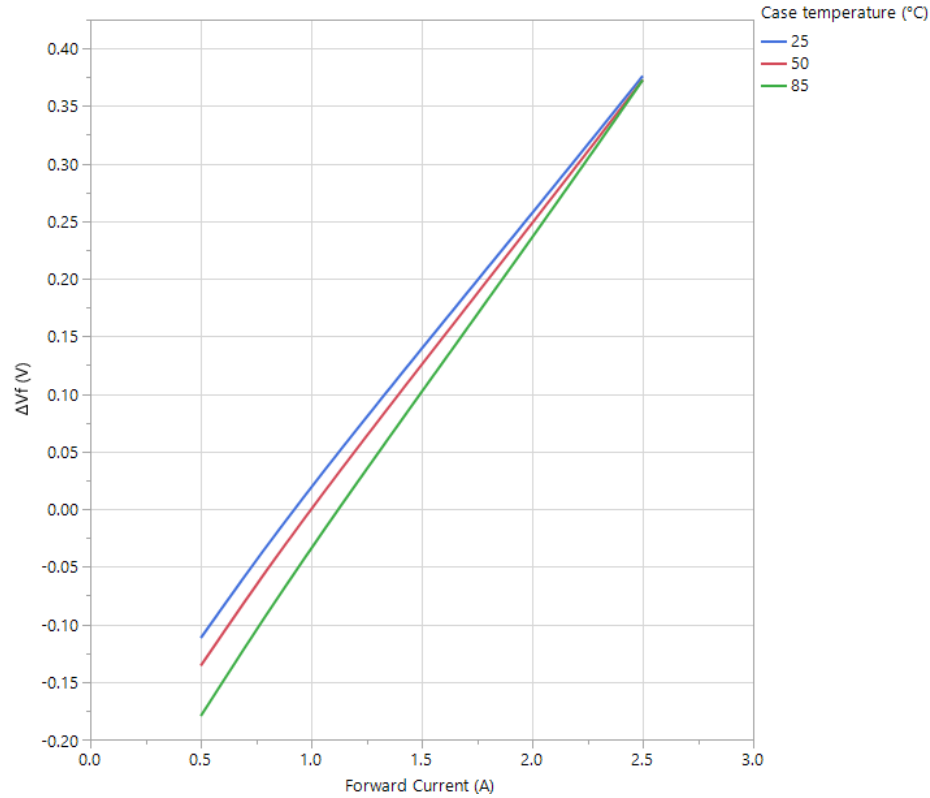
Figure 10: IR channel: change in forward voltage vs forward current (Normalized to at I_f = 1.0\text{A} and T_{\text{case}} = 50^\circ\text{C} )
