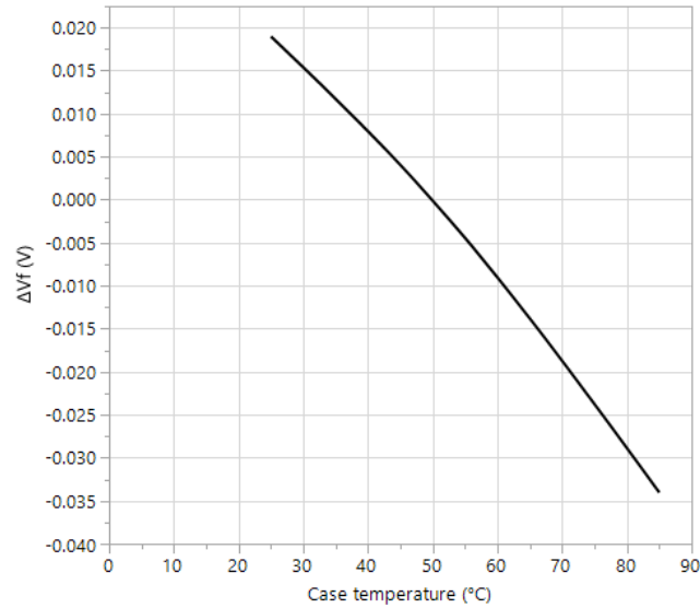
Figure 08: IR channel: change in forward voltage vs temperature (Measured at I_f = 1.0\text{A} and normalized at T_{\text{case}} = 50^\circ\text{C} )
