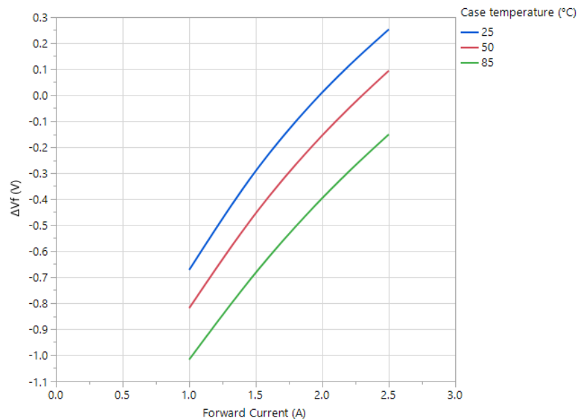
Figure 05: White channel: change in forward voltage vs forward current (Normalized to at I_f = 2.3\text{A} and T_{\text{case}} = 50^\circ\text{C} )
