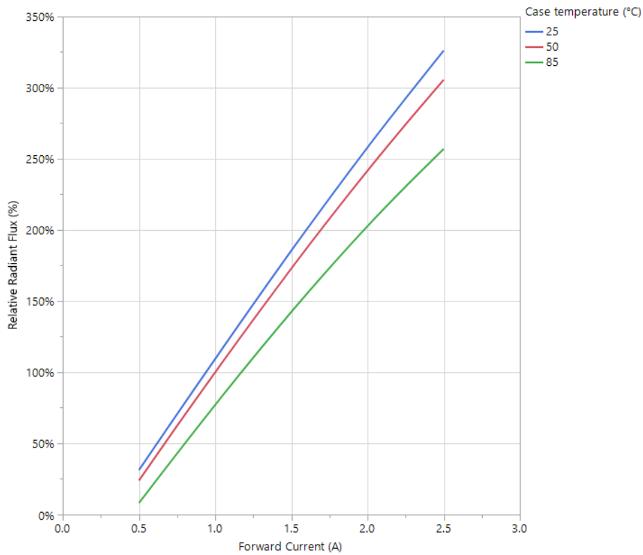
Figure 09: IR channel: relative radiant flux vs current (Normalized luminous flux at I_f = 1.0\text{A} and at T_{\text{case}} = 50^\circ\text{C} )
