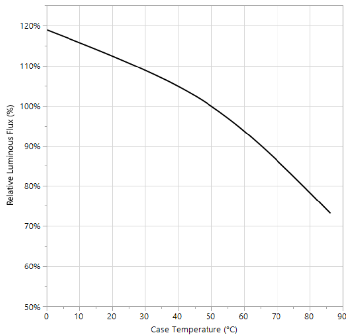
Figure 07: White channel: relative luminous flux vs case temperature (Normalized luminous flux at I_f = 2.3\text{A} and at T_{\text{case}} = 50^{\circ}\text{C} )
