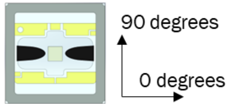
Figure 16: Orientation for near and far field plots
