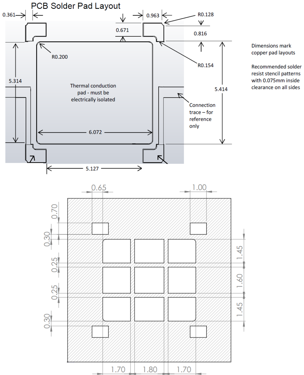
Figure 15: Recommended stencil mask design
