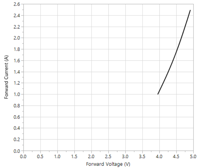
Figure 06: White channel: forward current vs forward voltage (Measured at T_{\text{case}} = 50^{\circ}\text{C} )
