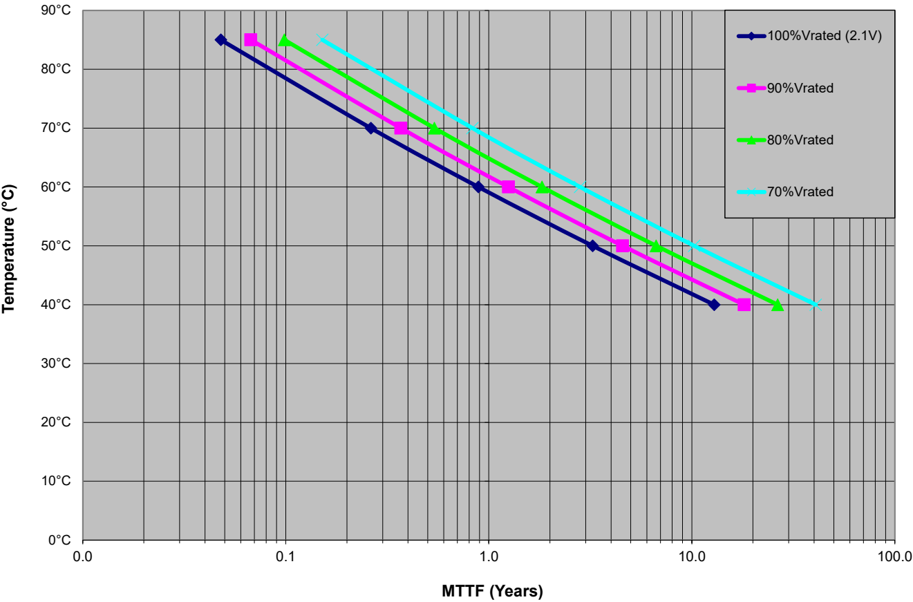
Expected Lifetime at Various Voltages PrizmaCap Series 2.1V Rated
